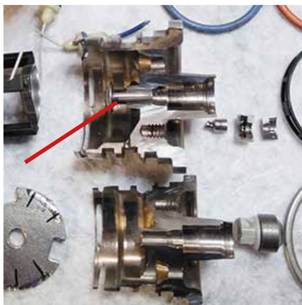
710-TGA2601; Rotax 850 2018- Rotax E-Tec Injector, open
